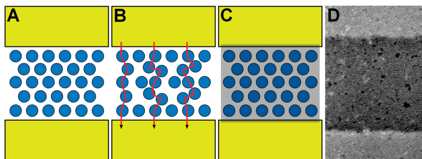
Figure 1. Possible mechanisms: (A) pristine, well ordered sample; (B) first possible conduction mechanism after annealing; shift of nanoparticles and enhanced conductivity through paths with shorter tunnel barriers; (C) second mechanism, carbonization of ligands; (D) SEM image of a CoPt nanoparticle monolayer deposited on a substrate structured with gold electrodes (the brighter parts).
