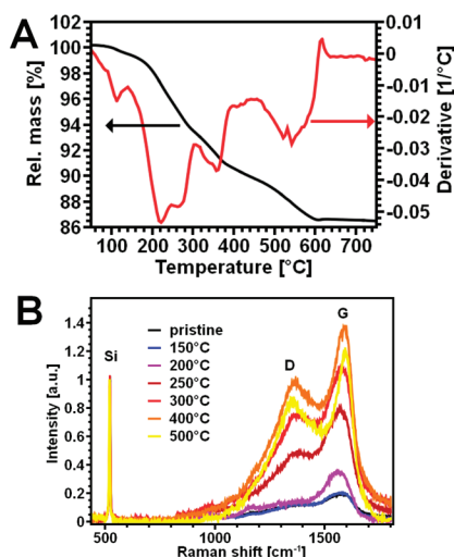
Figure 5. (A) Result of a thermo-gravimetric measurement (black) and the first derivative (red). The measurement was performed under nitrogen flow and with a heating rate of 20 °C/min. (B) Raman spectrum of a film annealed at different temperatures. The graphs are normalized to the silicon peak. The D and G peak intensity increases with rising annealing temperature. The G peak shifts to higher values with increasing annealing temperature.
