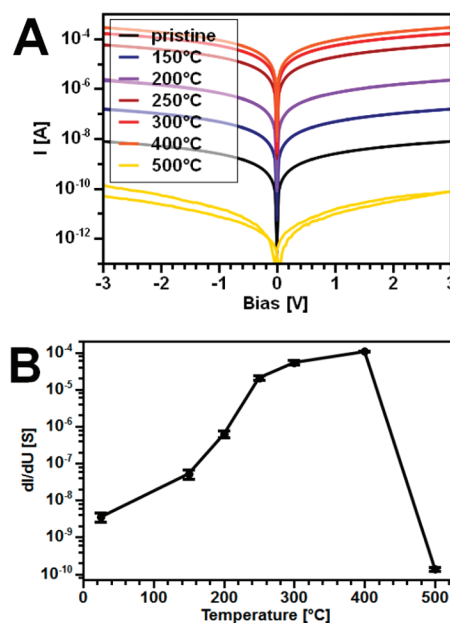
Figure 2. (A) I – V curves of a monolayer film, annealed at different temperatures and measured at room temperature. The conductivity increases with increasing annealing temperature up to 400 °C. (B) The conductivity at 3 V plotted against the annealing temperature.
