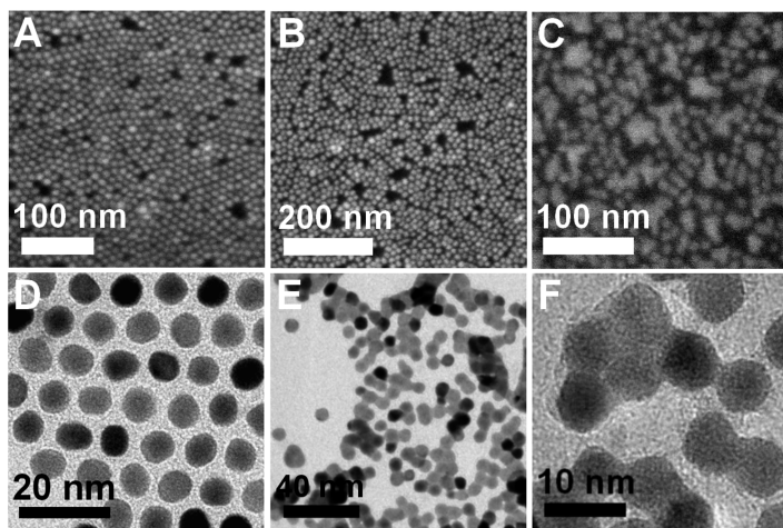
Figure 3. SEM images of monolayer films: (A) pristine, annealed at (B) 400 °C and (C) 500 °C. The annealed films show rifts and agglomerates. (D) TEM image of as-synthesized nanoparticles, (E) TEM images of particles annealed at 400 °C and (F) higher magnification.
