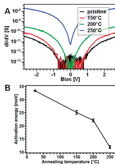
Figure 6. (A) Differential conductance of a pristine and annealed films at 4.3 K. The film annealed at 250 °C shows no sign of Coulomb blockade at 4.3 K and zero bias, while the untreated film clearly shows blockade below half a volt. The film treated at 200 °C shows reduced Coulomb blockade. (B) The activation energy decreases with increasing annealing temperature (at 2 V).
