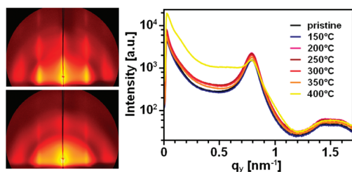
Figure 4. (Left) GISAXS pattern of thermally untreated particle film (top image) and a film annealed at 400 °C (bottom image). The structural change is well visible in the loss of clarity of the reflections. (Right) curves obtained by slicing the GISAXS pattern along the q_y axis.
